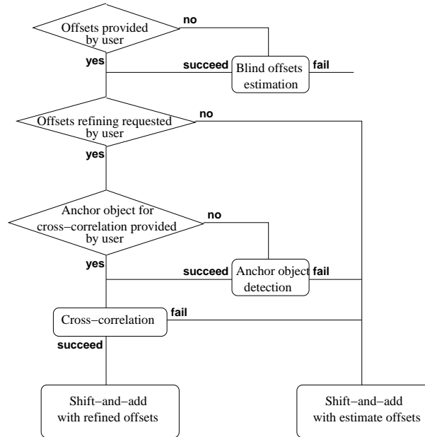
Figure 12: cpl_geom_img_offset_combine() behaviour
