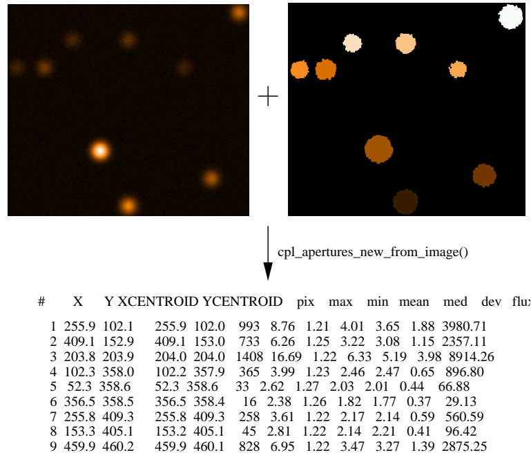
Figure 11: Usage of cpl_apertures_new_from_image()
