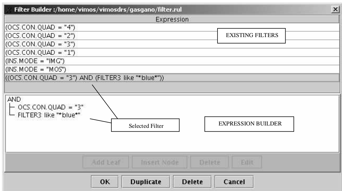
Figure 8: The Filter Builder window. In this example, rules are saved in the file filter.rul. It is possible to configure the file and its location through the File>Preferences panel. The upper panel shows a list of rules (Existing Rules), with the selected rule (highlighted in blue) displayed in the lower panel (Expression Builder).
