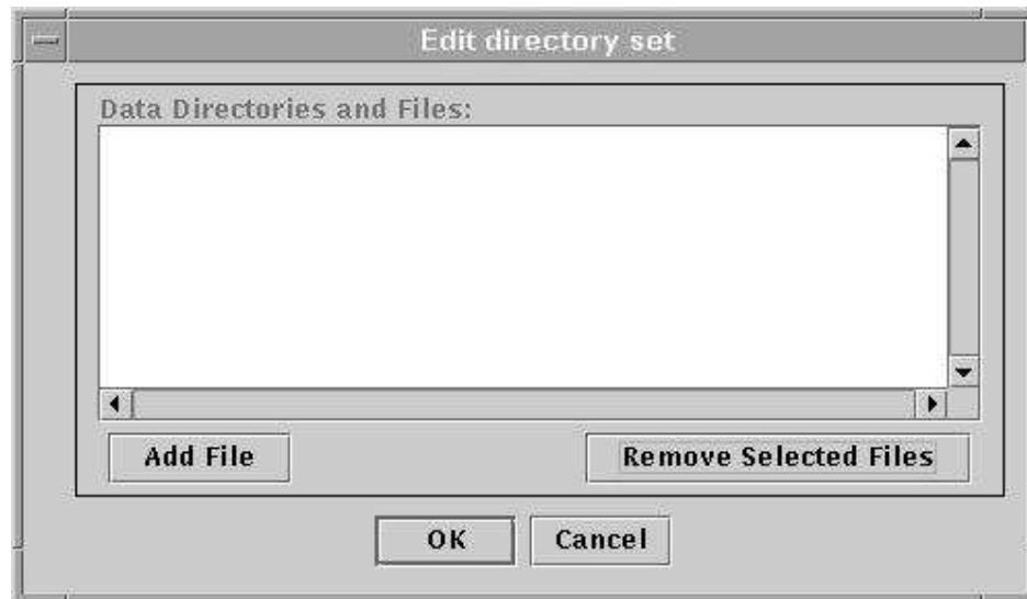
Figure 4: the Edit directory set window allows adding or removing directories/files to/from the Navigation Panel. In this example no files are loaded. Clicking on Add File opens a file chooser dialog for browsing and selecting files and directories.
