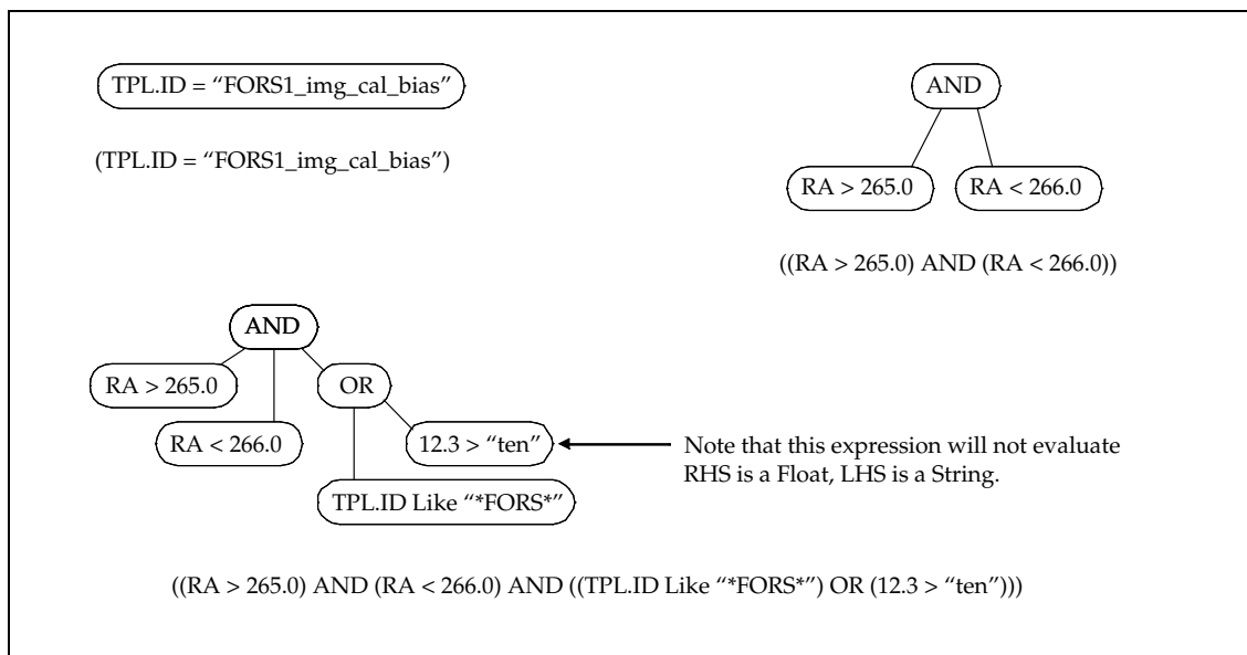
Figure 20: Expression Tree Examples
