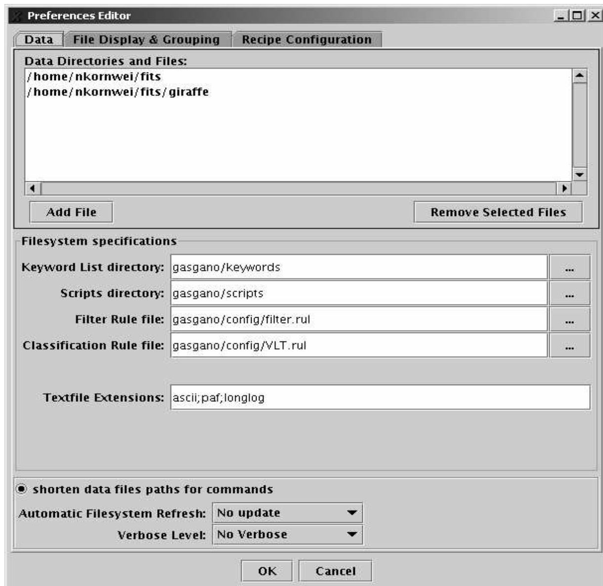
Figure 10: The Data panel under the Preferences Menu
