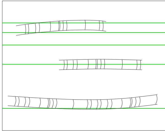
Figure 10.6.1: CCD rows may not cut the whole range of the raw arc lamp spectra, because the spectra are not read along their curvature. However, even incomplete portions of the searched pattern can be identified by the pattern-matching algorithm.
