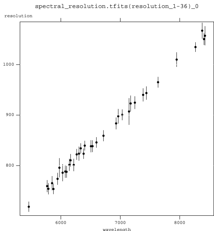
Figure 9.8.6: Resolution vs. wavelength in a SPECTRAL_RESOLUTION_MXU table derived from a FORS2 MXU 600RI arc lamp exposure.
