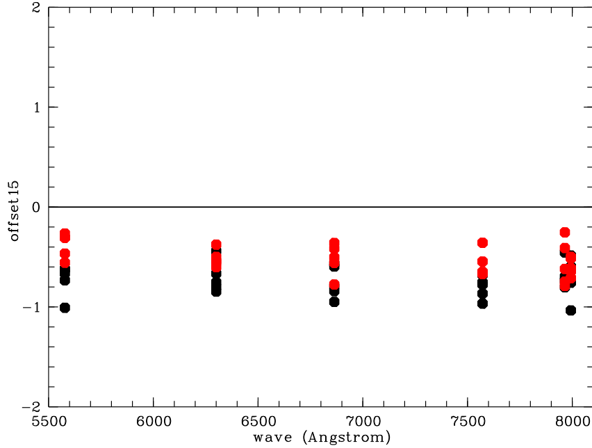
Figure A.4.1: Systematic sky line offsets (in pixel) from day-calibration expectation, observed in a FORS2 MXU 600RI scientific exposure. The offsets from all slits are plotted, black and red points belonging to slits from the upper and lower part of the CCD. All offsets are systematically negative, and therefore a sky alignment of the wavelength solution is due. Offsets depending on the slit position on the CCD, as shown by the different distribution of black and red points in figure, indicate that the scientific exposure is not just translated (e.g., by flexures) but also rotated with respect to day calibrations.
