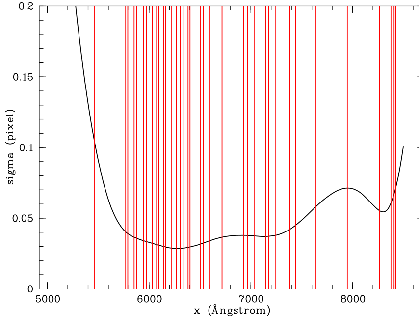
Figure 9.8.2: Montecarlo simulation of wavelength calibration model accuracy (from FORS2/MXU 600RI calibration lamp). The curve describes the changing accuracy (in pixel), given at 1- \sigma confidence level. The vertical lines indicate the positions of the used reference arc lamp lines. It is possible to see that, as expected, the calibration is more accurate where the density of lines is higher. The accuracy of the model degrades rapidly at the blue and red ends of the spectrum, where uncertainties due to overfitting and extrapolation are greater.
