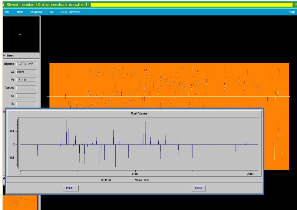
Figure 9.8.3: DISP_RESIDUAL_MXU from a FORS2 MXU 600RI arc lamp calibration. In the foreground is a plot of the residuals from one image row.
