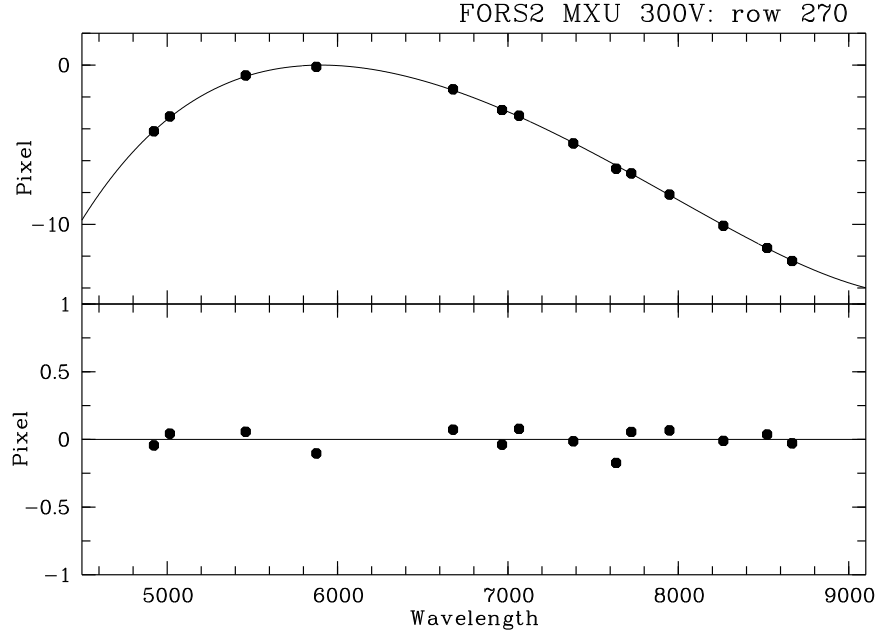
Figure 9.8.1: Top panel: deviation of the identified peaks from the linear term of the 270th fitting polynomial (column d270 of the DISP_RESIDUALS_TABLE_MXU). The solid line is the polynomial model with the linear term subtracted, drawn from row 270 of the DELTA_IMAGE_MXU product. Bottom panel: fit residuals of the identified peaks (identical to the residuals recorded at row 270 of the DISP_RESIDUALS_MXU image).
