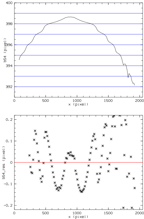
Figure 9.8.7: Systematic residuals of curvature model (from a FORS2 MXU 600B flat field exposure).
