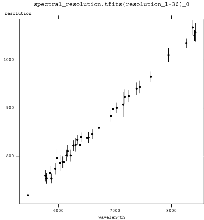
Figure 9.8.6: Resolution vs. wavelength in a SPECTRAL_RESOLUTION_MXU table derived from a FORS2 MXU 600RI arc lamp exposure.
