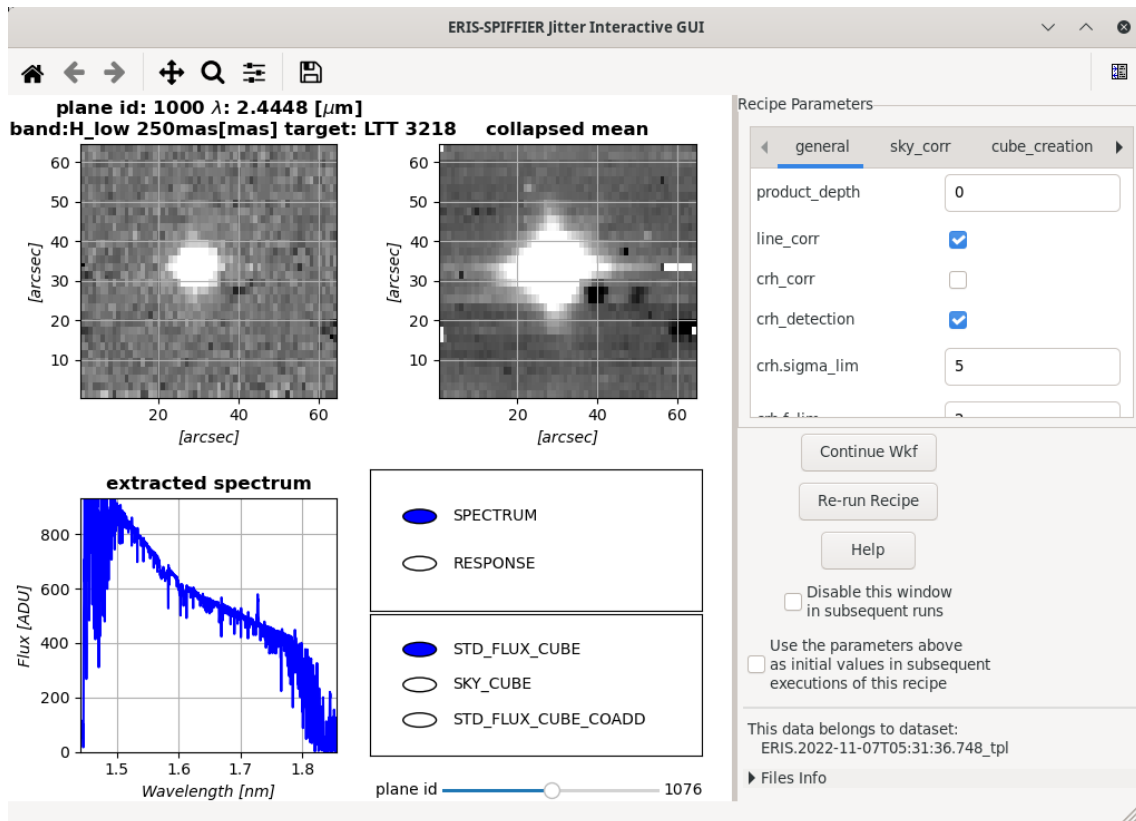
Figure 9.8: The interactive window to edit parameters of recipe eris_ifu_stdstar on flux STD star data.
