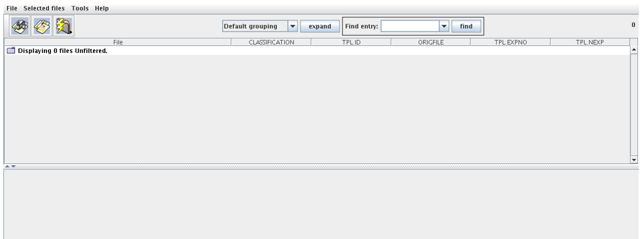
Figure 4.2.1: The Gasgano main window.
