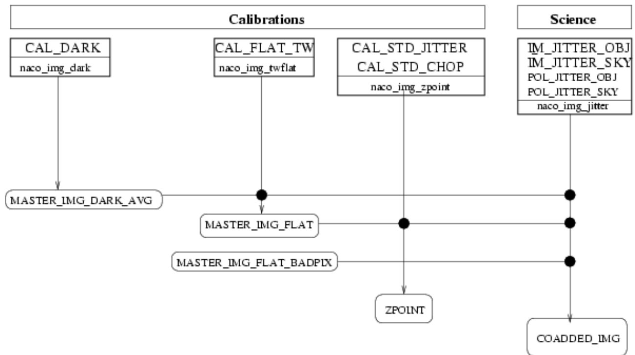
Figure 8.3.1: NACO Association Map in imaging mode. The rectangles indicate raw data, and specifies the matching recipe, while rounded rectangles indicate calibration.
