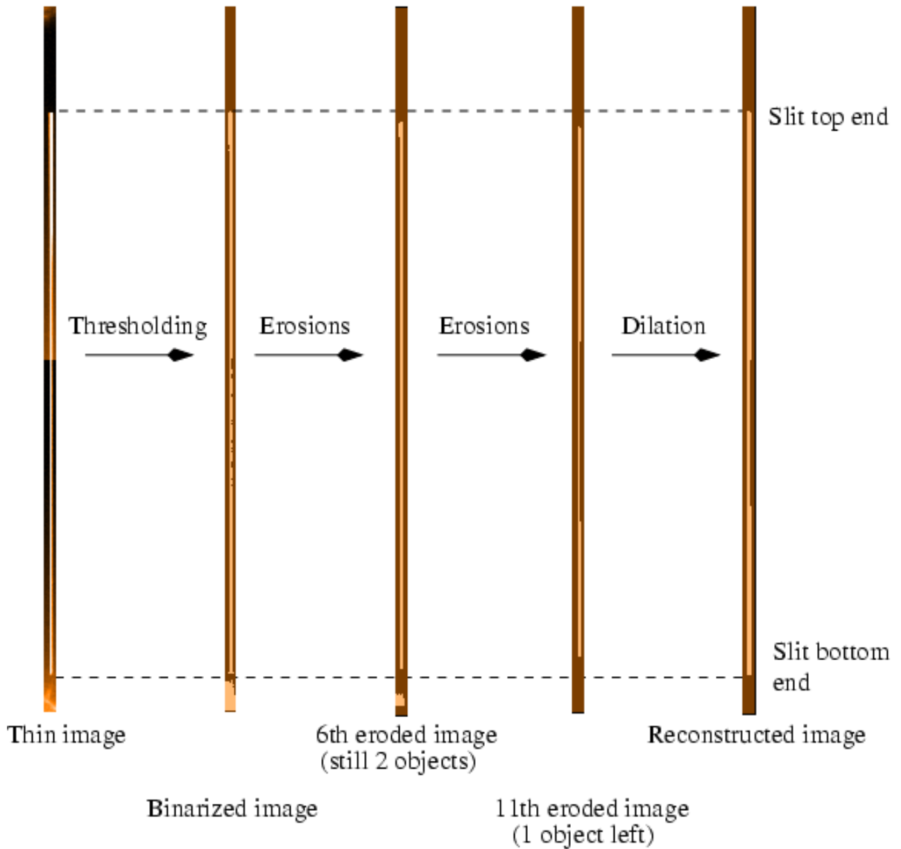
Figure 10.1.2: Slit detection.
