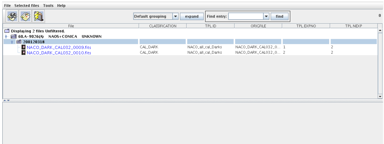
Figure 4.2.3: The Gasgano main window with the example FITS files loaded.
