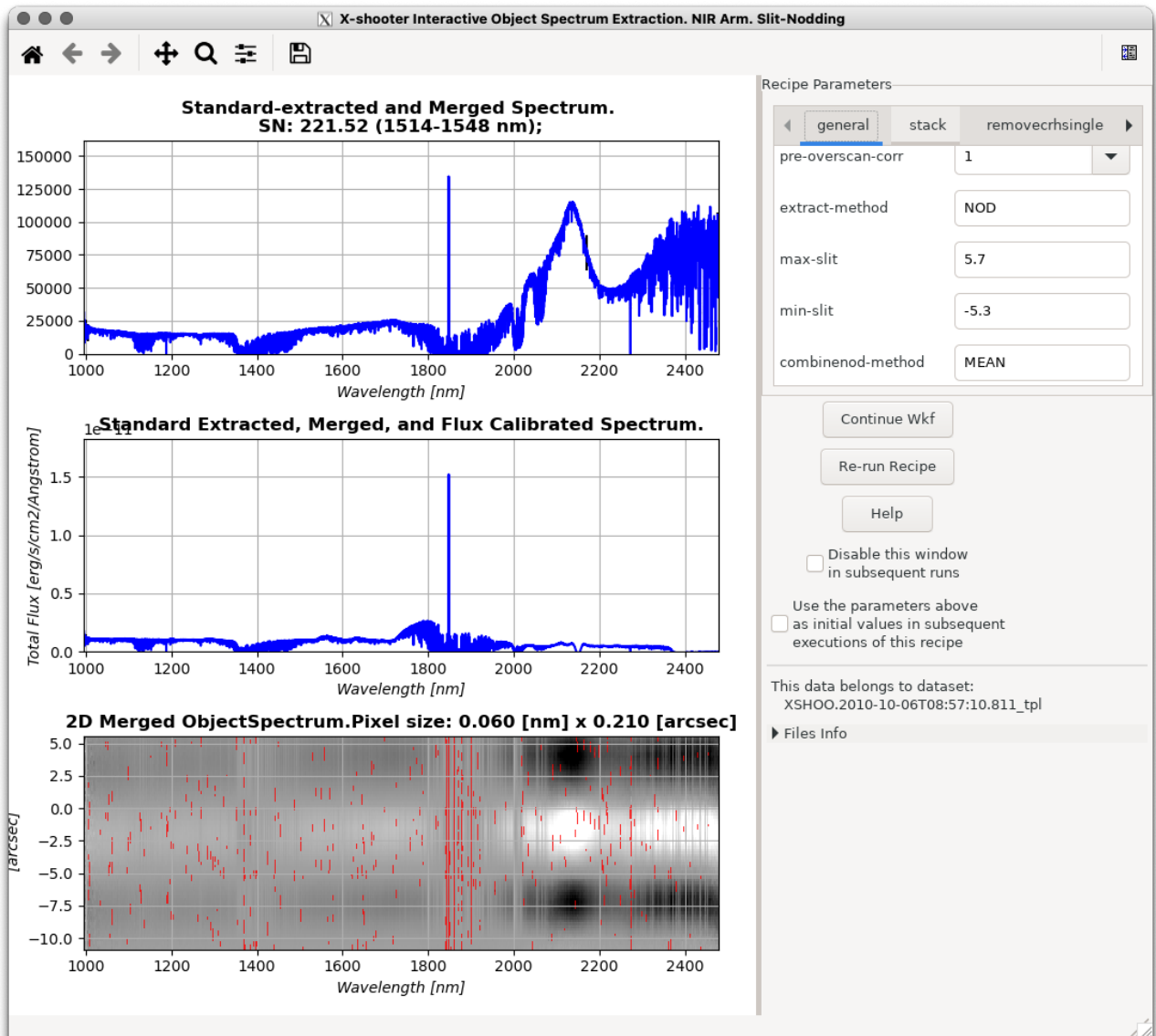
Figure 7.4: The interactive window for the Science Reduction actor for the recipe xsh_scired_slit_nod . The weird shape of the flux-calibrated spectrum in the middle panel is due to problems with offset mode flux standard star data (see Sect. 7.5 for more details).
