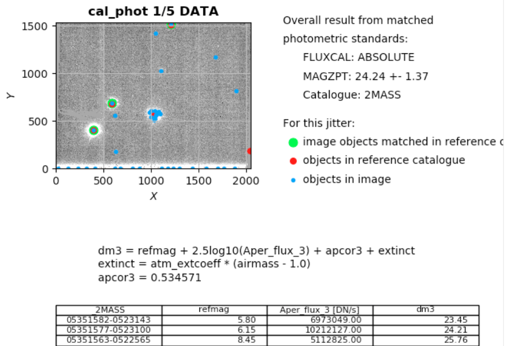
Figure 11.17: Workflow display of a jitter image of Theta Ori that contains objects 'matched' (green rims) with the photometric reference catalogue.
