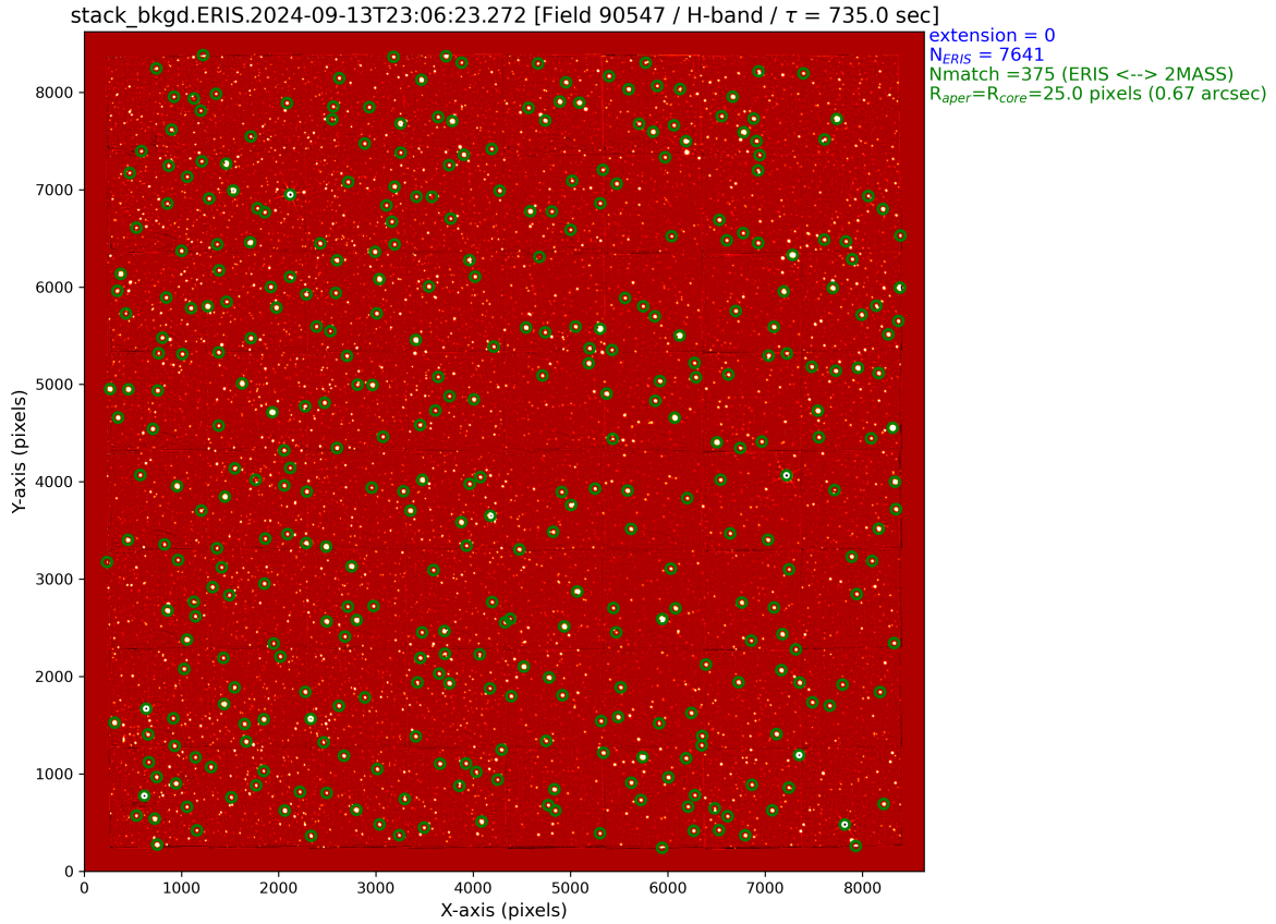
Figure 8.5: The pipeline combined mosaic of 49 ERIS-NIX H -band images of the S90547 2MASS touchstone field. The 2MASS sources used in the determination of the field zeropoint are shown in green apertures.
