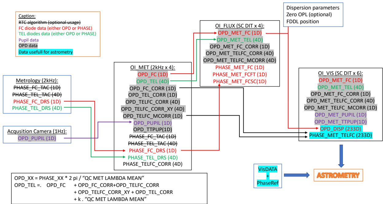
Figure 9.5: The data flow of the metrology, starting from the phase extracted from the metrology voltage, to the final products OPD_DISP and PHAS_MET_TEFRC
