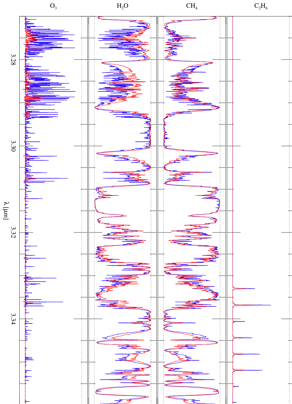
Figure C.2: Influence of individual molecules as a function of wavelength: same as Figure C.1, but for the CRIFES test data wavelength regime.
