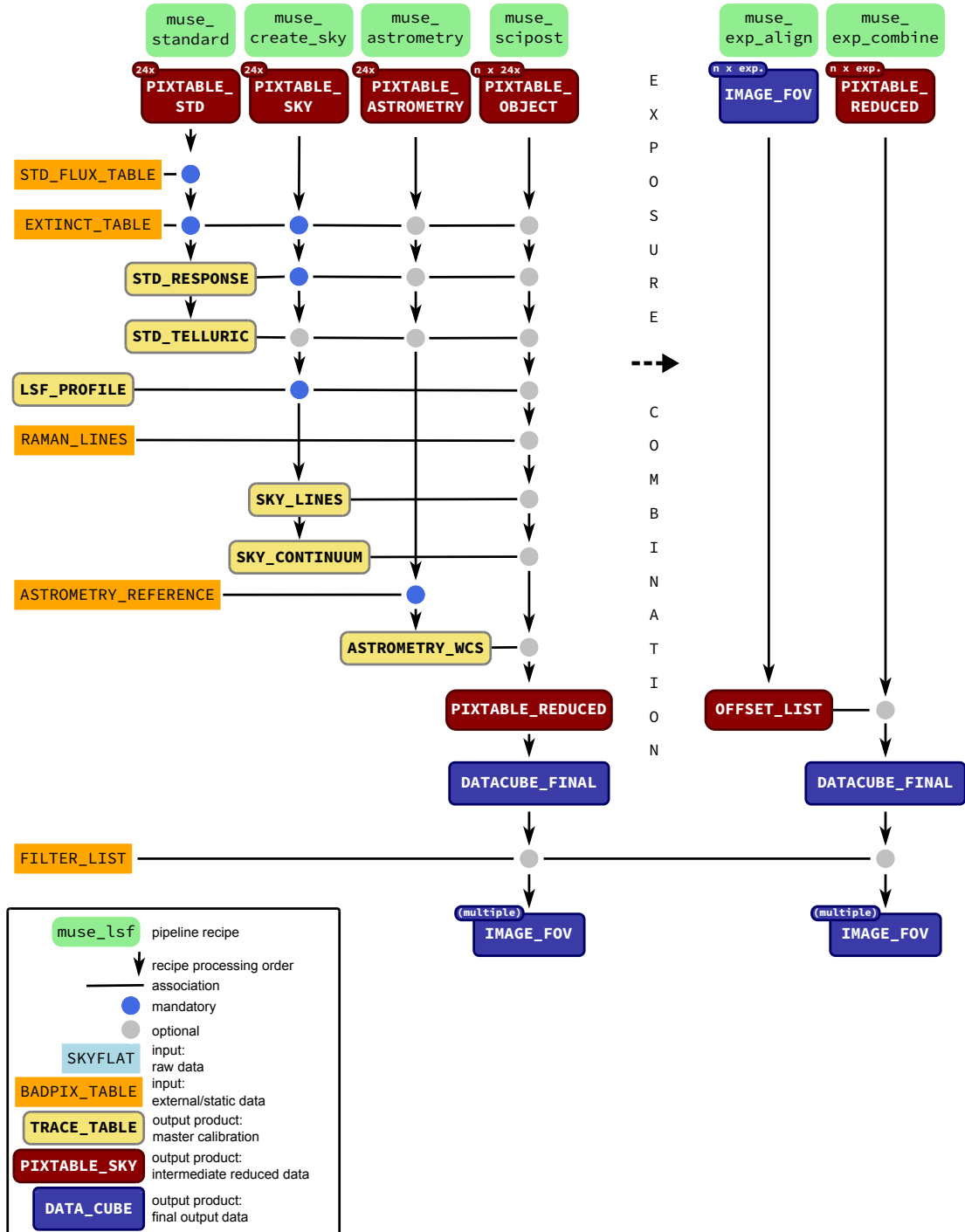
Figure 2.3: The second stage of the MUSE data reduction cascade. These recipes start from the output of the pre-processing recipe muse_scibasica and combine the data from all 24 IFUs into a single, fully reduced and calibrated data cube. The two recipes on the right side show the (optional) alignment of several exposures and their combination as an optional, final processing step. Again the “Association map” indicates the required and the optional input for each of the recipes.
