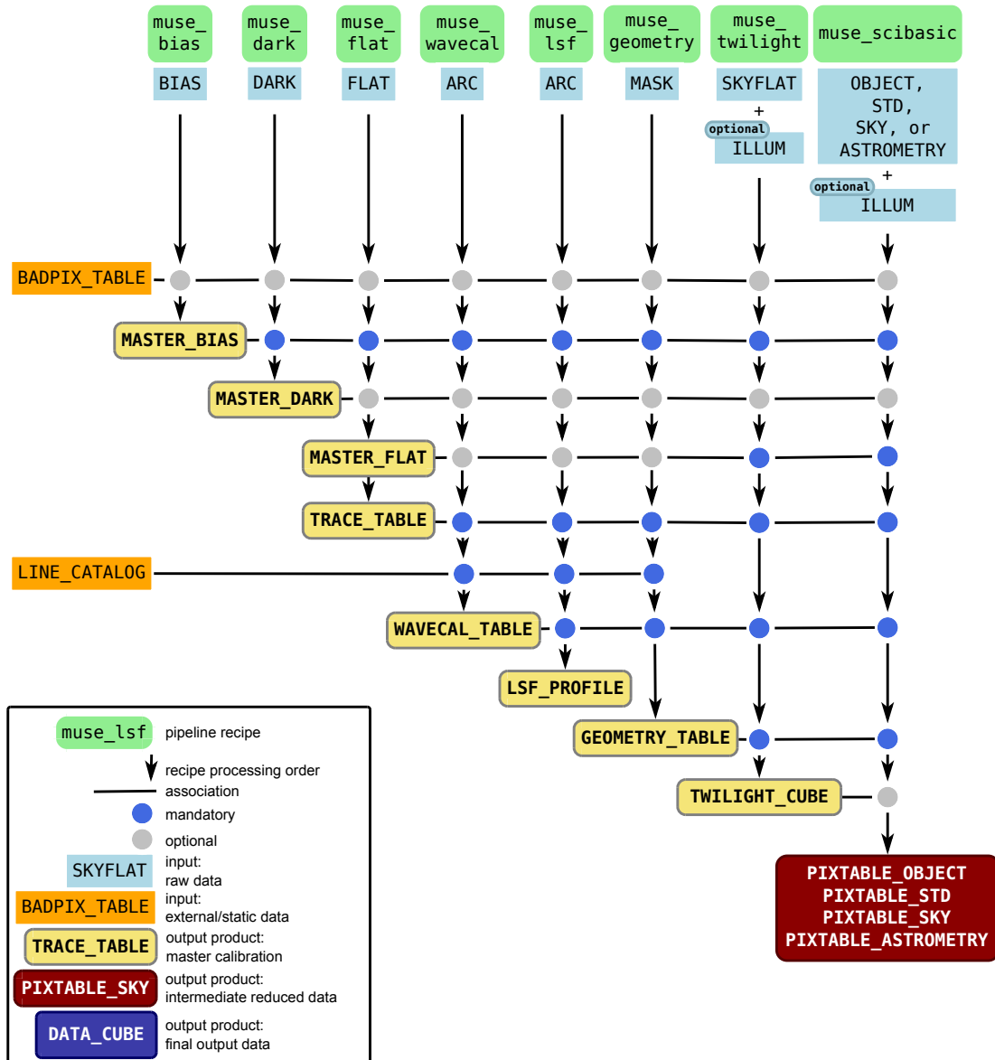
Figure 2.2: The first stage of the MUSE data reduction cascade. It shows the basic calibration recipes and the pre-processing recipe muse_scibasic, together with the “Association map” indicating the required and the optional input for each of the recipes.
