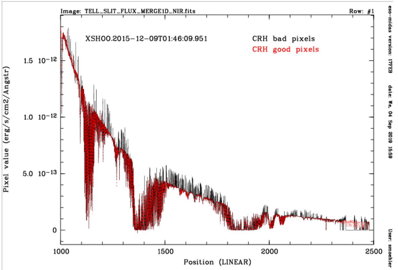
Figure 8.2: NIR standard star spectrum obtained in very good seeing processed with pipeline default parameters (black) and setting the decode-bp parameter to decode-bp = decode-bp - 32 to accept detected CRHs as good pixels (red).
