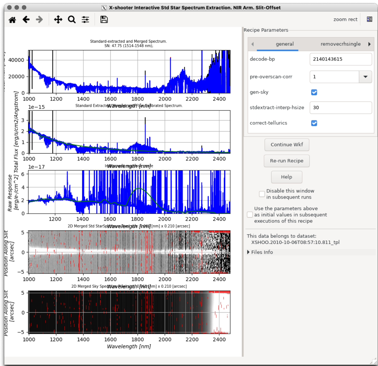
Figure 7.9: Interactive window of the Instrument Response actor for the recipe xsh_respon_slit_offset. The extracted spectrum in the top panel shows clear evidence for sky lines being brighter in the sky frame than in the standard star frame. The weird shape of the response curve is due to these problems with the sky correction of the flux standard star data. Pls note that we have zoomed on the Y axis of the middle panel to make appear this defect.
