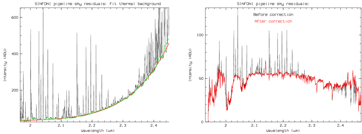
Figure 11.15: The fit of a sky spectrum is shown on the left panel. The sky background (black) is first smoothed (green) and then fit by a Boltzmann function (red). On the right panel we compare un-corrected (black) and corrected (red) sky subtracted object spectra. Rotational transitions affect the spectrum quality by only 1-5%. Not only can one see 1-0S(1) at 2.12 \mu\text{m} and \text{Br}_\gamma at 2.17 \mu\text{m} , but now the H2 1-0Q(1) and 1-0Q(3) emission lines are clearly seen longward of 2.4 \mu\text{m} , and several CO band-heads are also visible at 2.3-2.4 \mu\text{m} .
