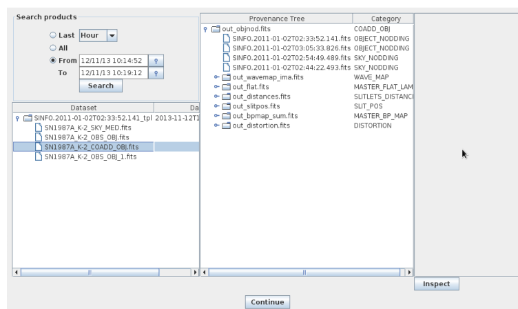
Figure 4.0.4: The Provenance Explorer shows all datasets reduced in previous executions together with the full reduction chain for all the pipeline products.
