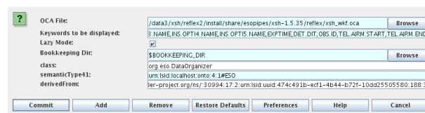
Figure A.1: Parameter to change for the OCA file, used for classification, grouping and association of data.
