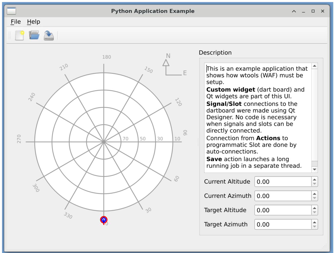
Fig. 48: Python Application Example - GUI design to achieve in this example.
