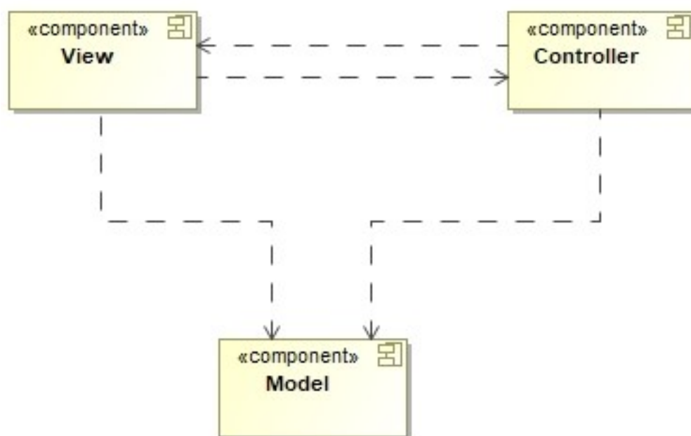
Fig. 7: MVC Component Diagram
