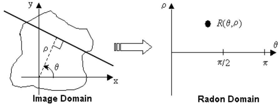
Figure 17: The Radon Transform
