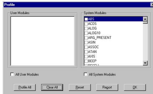
Figure 12-4: Profile Dialog
